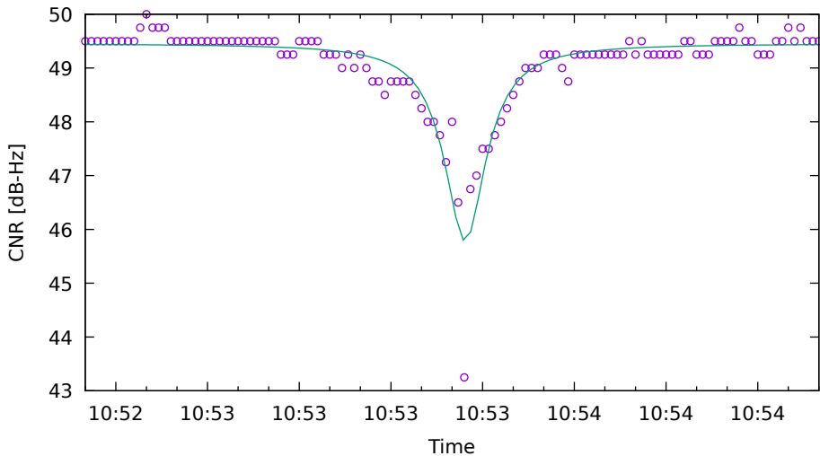
CNR fit for G09 on SamsungS20 - drive 8 (DOY263)
