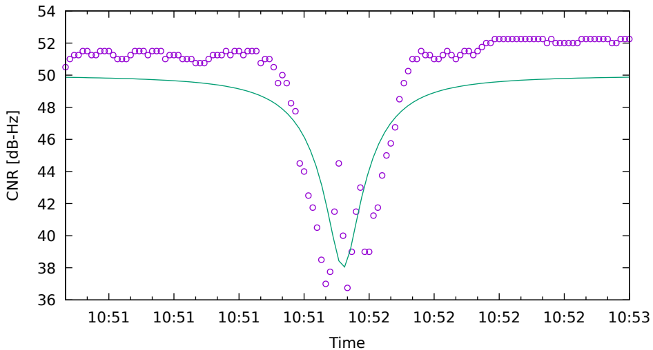
CNR fit for G17 on SamsungS20 - drive 7 (DOY263)
