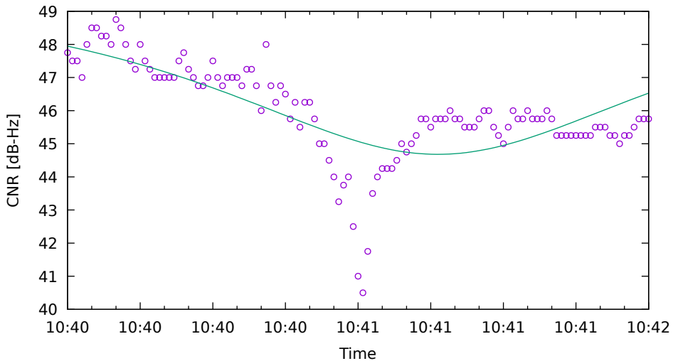
CNR fit for G21 on SamsungS20 - drive 1 (DOY263)
