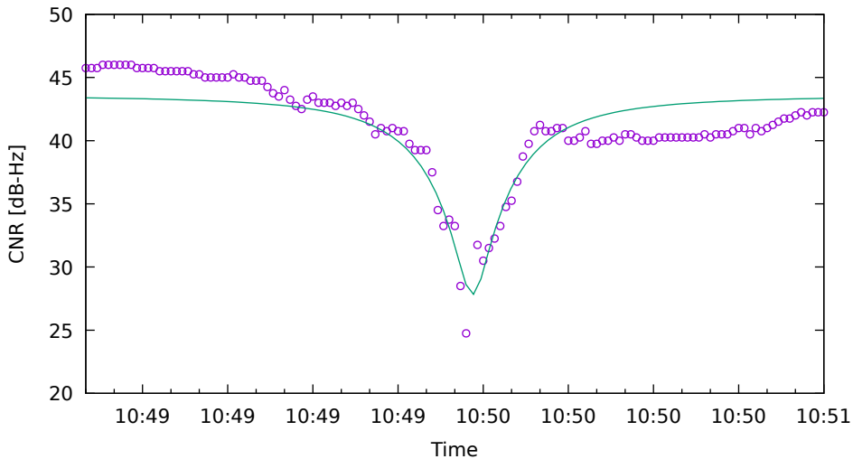
CNR fit for G21 on SamsungS20 - drive 6 (DOY263)
