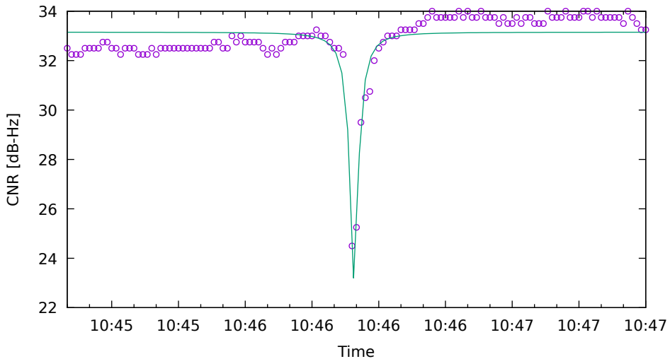
CNR fit for C09 on Xiaomi11T - drive 4 (DOY263)
