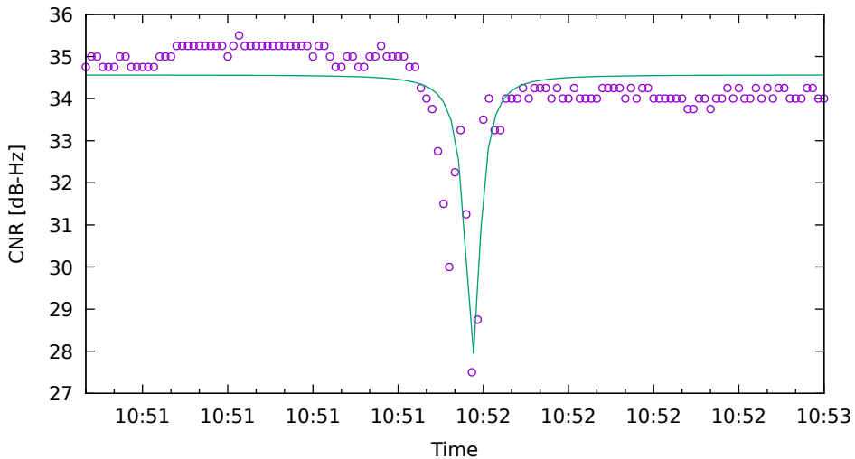
CNR fit for C09 on Xiaomi11T - drive 7 (DOY263)
