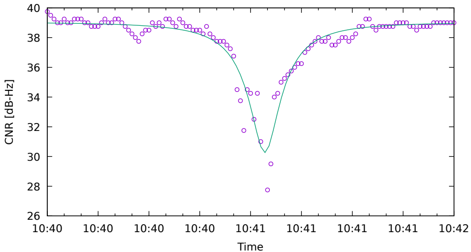
CNR fit for C11 on Xiaomi11T - drive 1 (DOY263)
