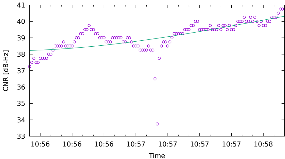
CNR fit for C11 on Xiaomi11T - drive 10 (DOY263)
