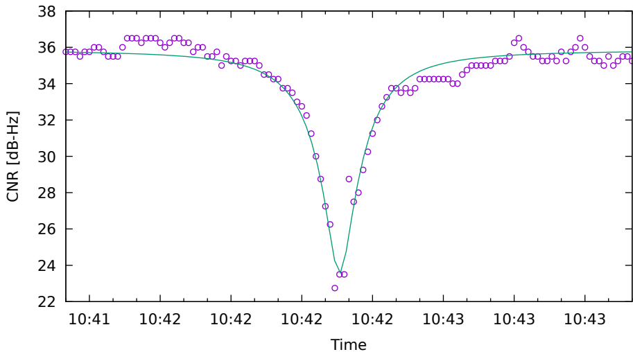
CNR fit for C21 on Xiaomi11T - drive 2 (DOY263)
