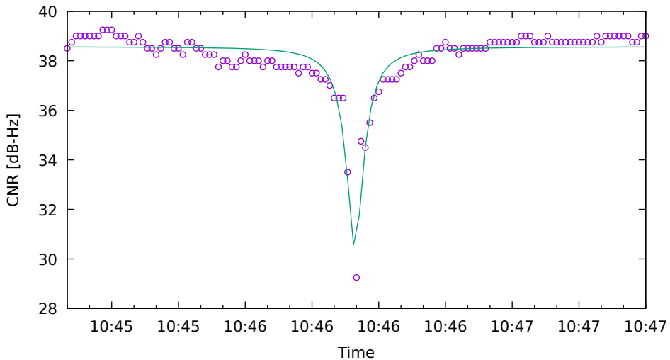
CNR fit for C21 on Xiaomi11T - drive 4 (DOY263)
