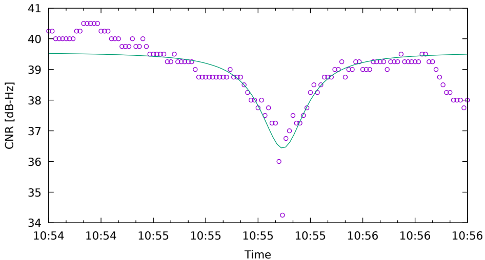
CNR fit for C21 on Xiaomi11T - drive 9 (DOY263)
