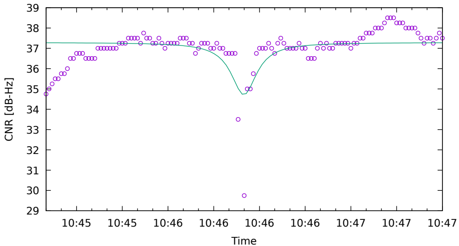
CNR fit for C26 on Xiaomi11T - drive 4 (DOY263)
