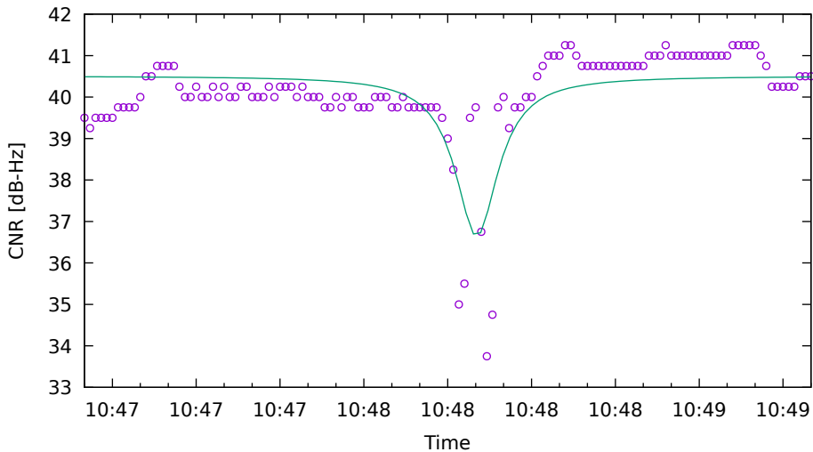
CNR fit for C28 on Xiaomi11T - drive 5 (DOY263)
