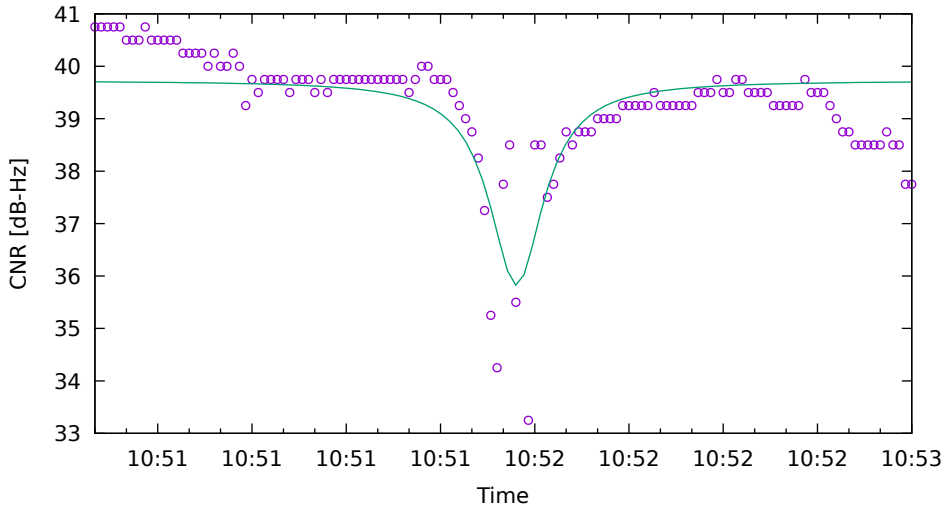
CNR fit for C28 on Xiaomi11T - drive 7 (DOY263)
