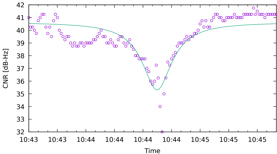
CNR fit for E04 on Xiaomi11T - drive 3 (DOY263)
