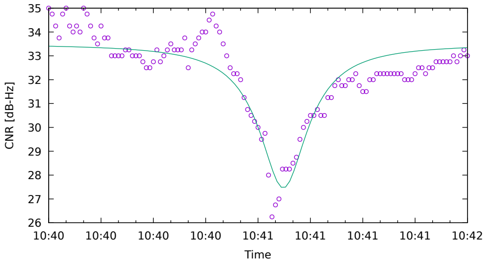
CNR fit for E33 on Xiaomi11T - drive 1 (DOY263)
