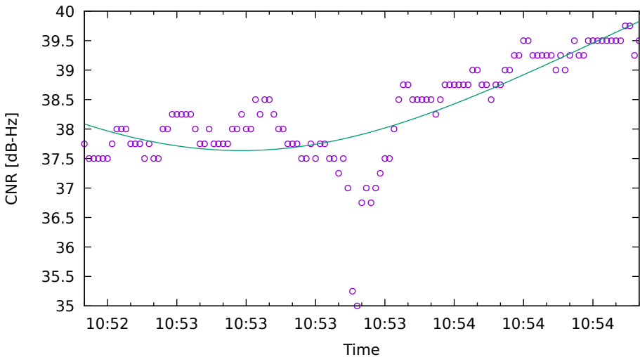
CNR fit for E33 on Xiaomi11T - drive 8 (DOY263)
