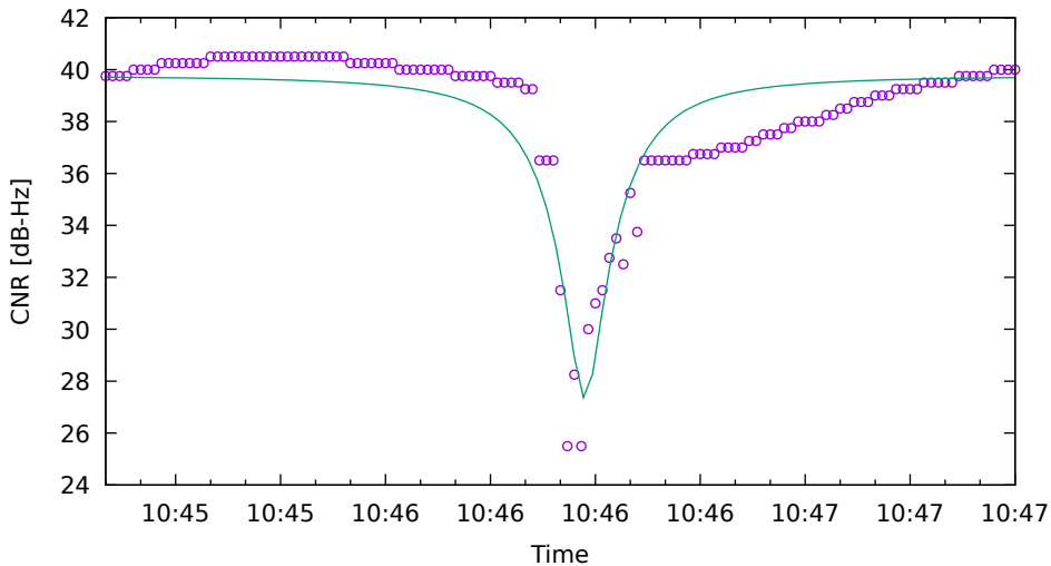
CNR fit for G03 on Xiaomi11T - drive 4 (DOY263)
