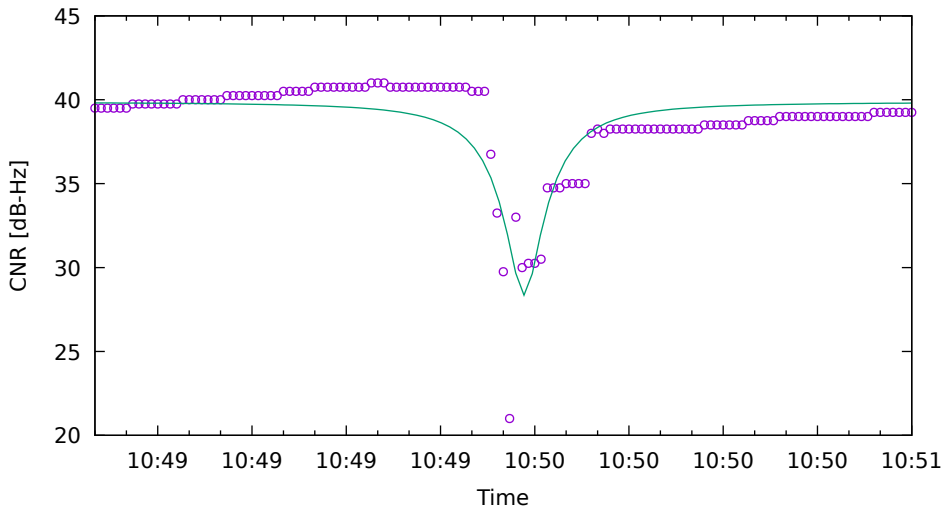
CNR fit for G03 on Xiaomi11T - drive 6 (DOY263)
