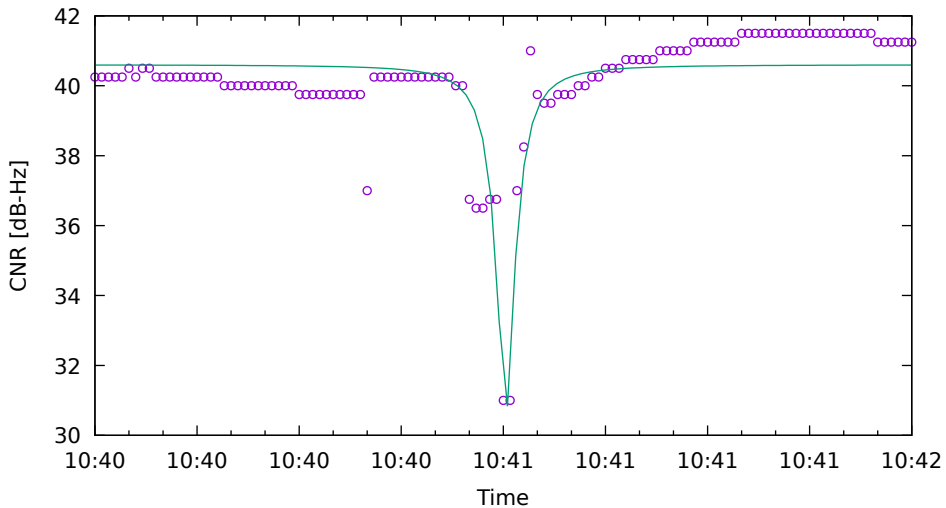
CNR fit for G19 on Xiaomi11T - drive 1 (DOY263)
