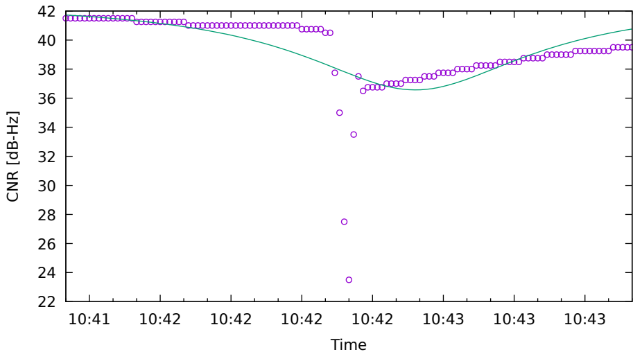
CNR fit for G19 on Xiaomi11T - drive 2 (DOY263)
