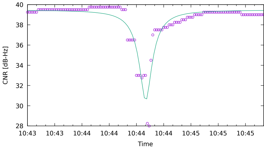
CNR fit for G19 on Xiaomi11T - drive 3 (DOY263)
