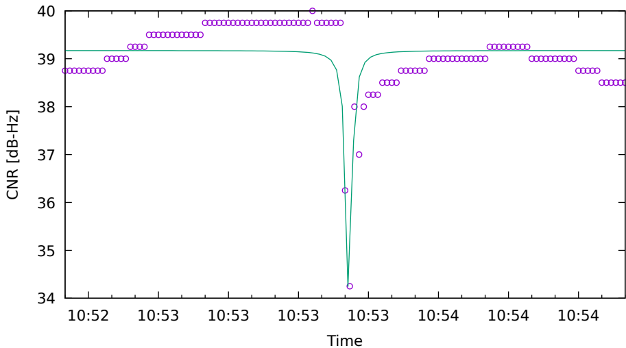
CNR fit for G21 on Xiaomi11T - drive 8 (DOY263)
