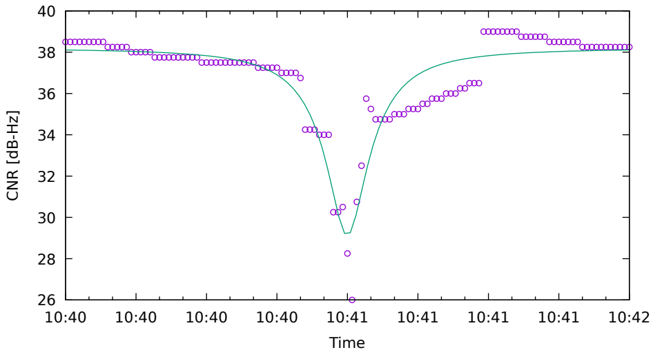
CNR fit for G31 on Xiaomi11T - drive 1 (DOY263)
