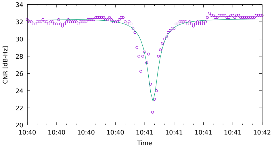
CNR fit for C09 on XiaomiMi8 - drive 1 (DOY263)
