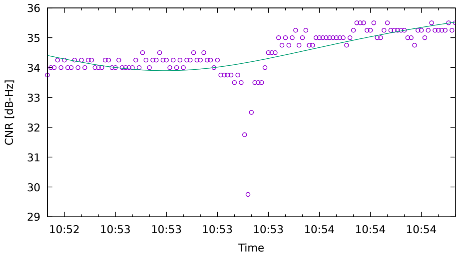
CNR fit for C09 on XiaomiMi8 - drive 8 (DOY263)
