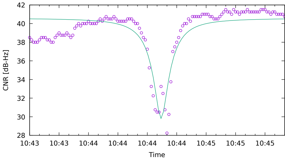
CNR fit for C11 on XiaomiMi8 - drive 3 (DOY263)
