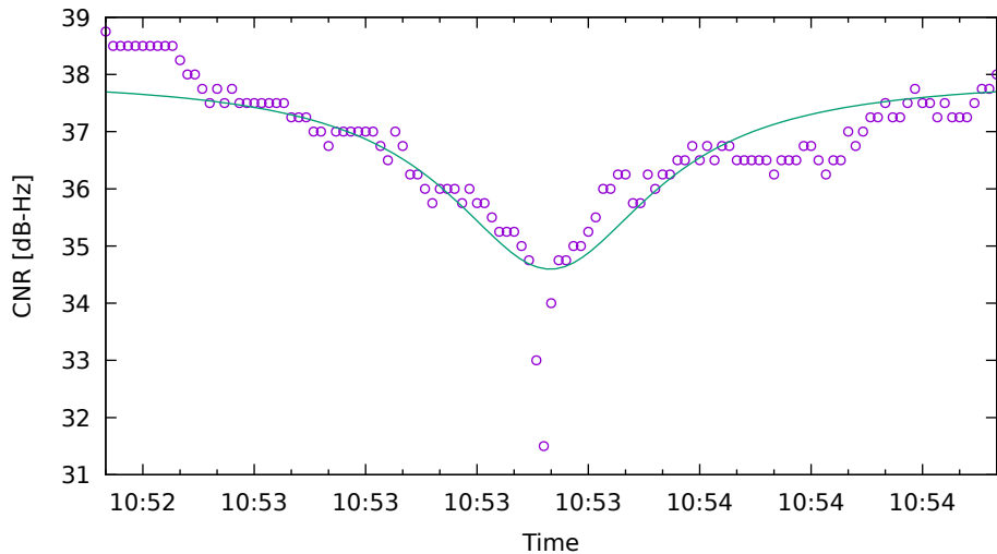
CNR fit for C11 on XiaomiMi8 - drive 8 (DOY263)
