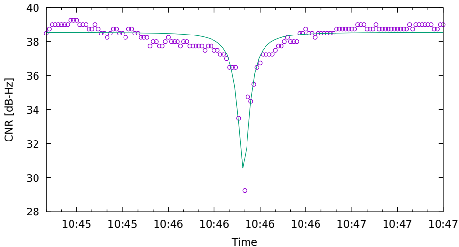
CNR fit for C21 on XiaomiMi8 - drive 4 (DOY263)
