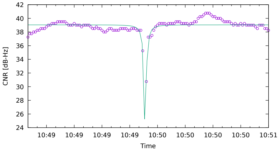
CNR fit for C26 on XiaomiMi8 - drive 6 (DOY263)
