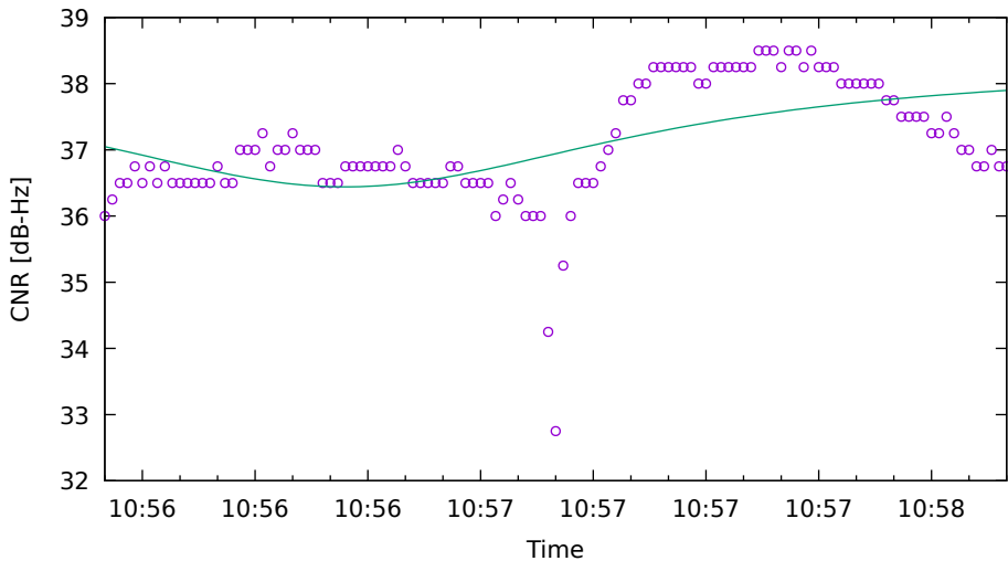
CNR fit for C28 on XiaomiMi8 - drive 10 (DOY263)
