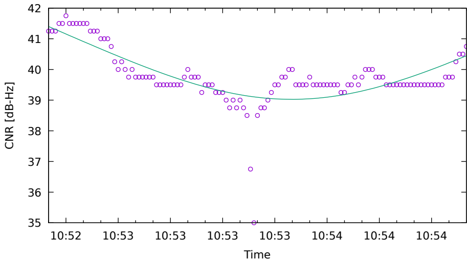
CNR fit for C33 on XiaomiMi8 - drive 8 (DOY263)
