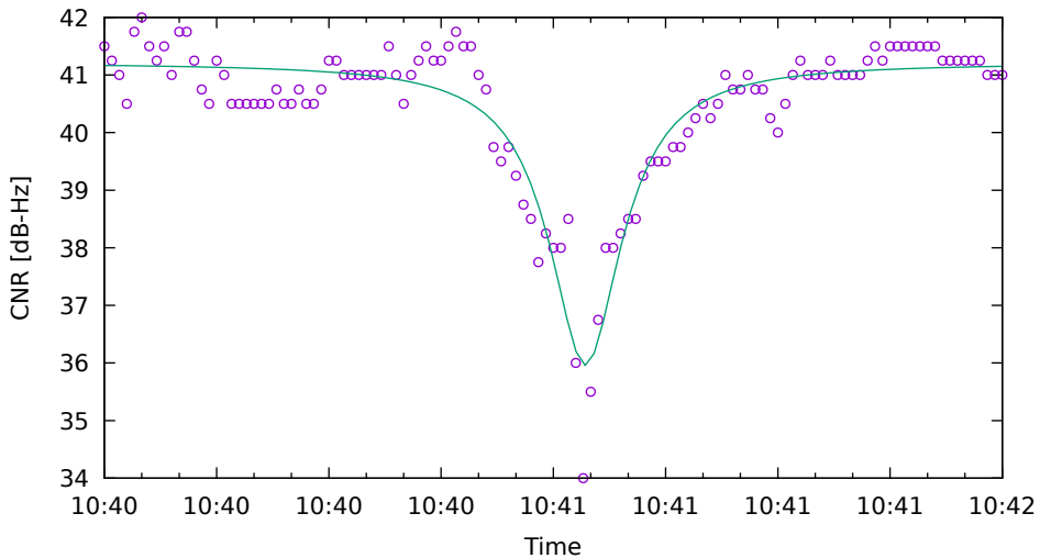
CNR fit for E04 on XiaomiMi8 - drive 1 (DOY263)
