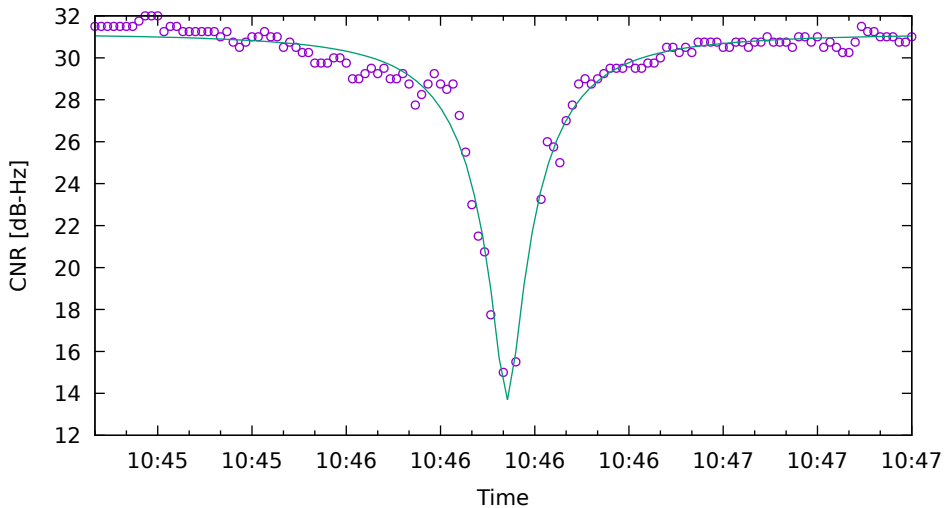
CNR fit for E19 on XiaomiMi8 - drive 4 (DOY263)
