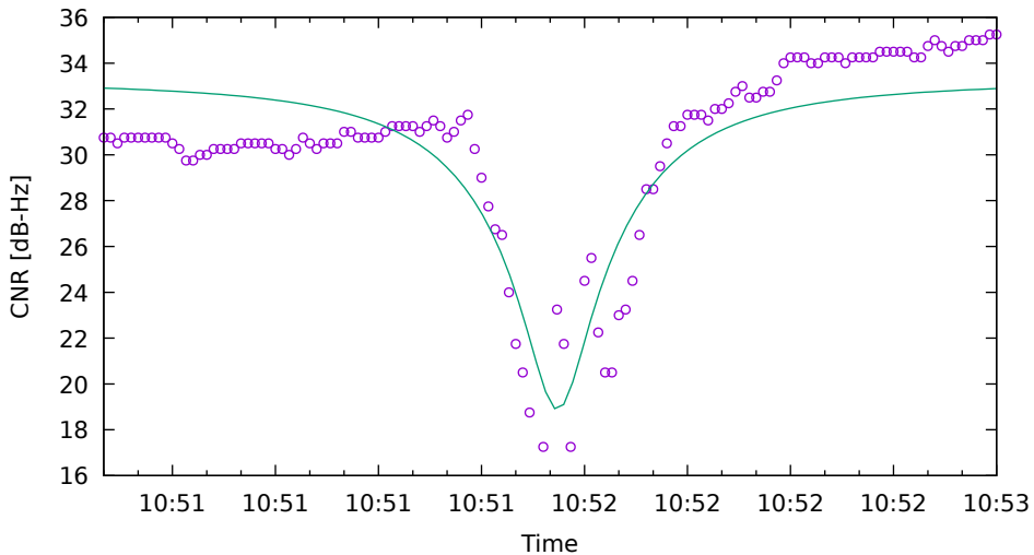
CNR fit for E19 on XiaomiMi8 - drive 7 (DOY263)
