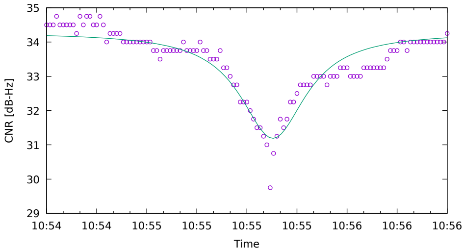
CNR fit for E19 on XiaomiMi8 - drive 9 (DOY263)
