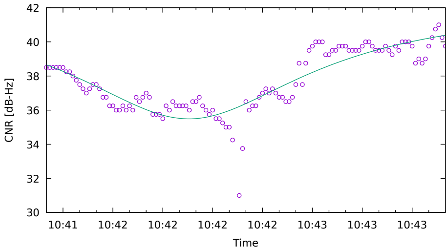
CNR fit for G01 on XiaomiMi8 - drive 2 (DOY263)
