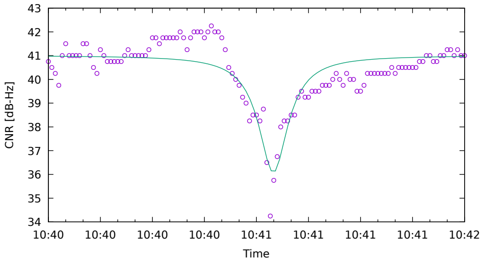
CNR fit for G03 on XiaomiMi8 - drive 1 (DOY263)
