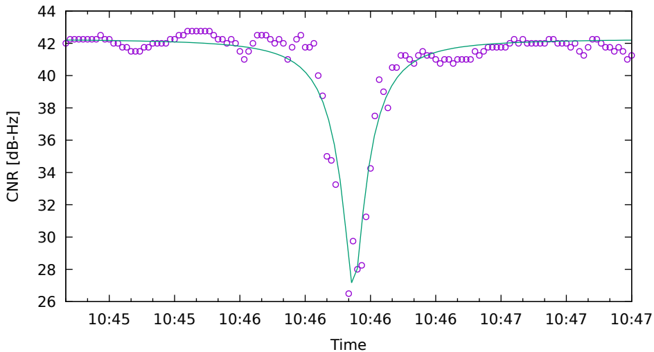
CNR fit for G03 on XiaomiMi8 - drive 4 (DOY263)
