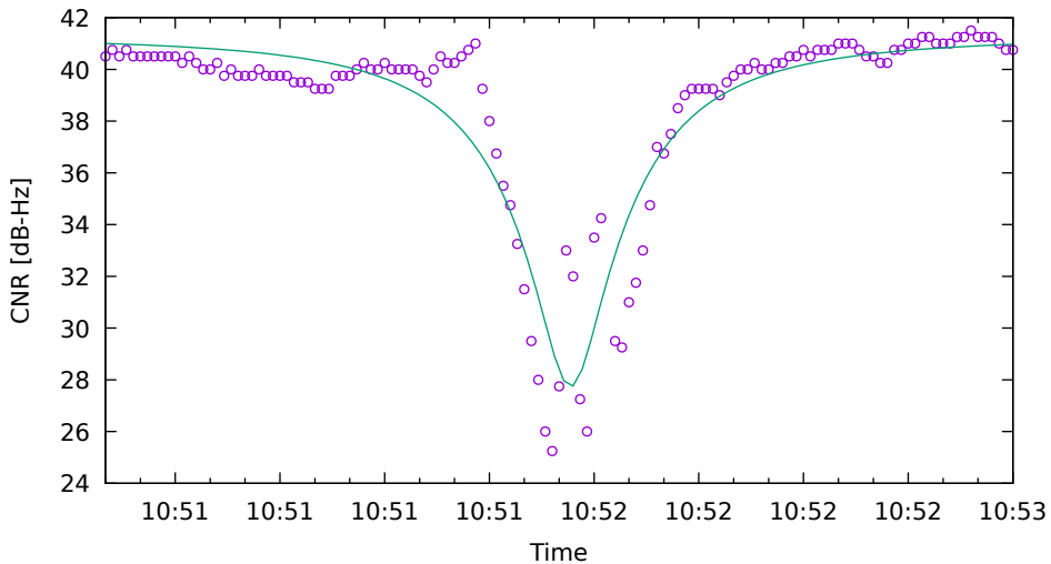
CNR fit for G03 on XiaomiMi8 - drive 7 (DOY263)
