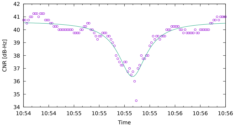
CNR fit for G03 on XiaomiMi8 - drive 9 (DOY263)
