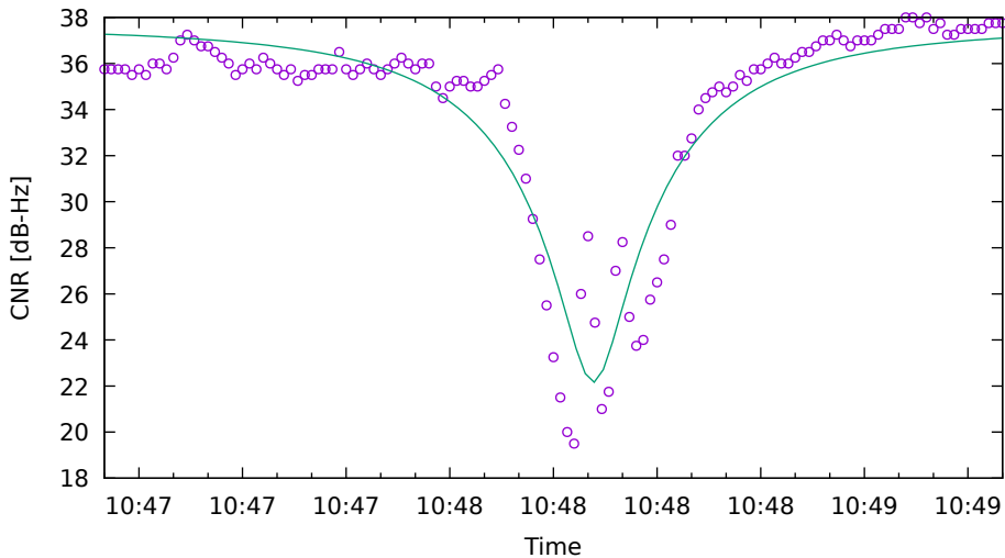
CNR fit for G04 on XiaomiMi8 - drive 5 (DOY263)
