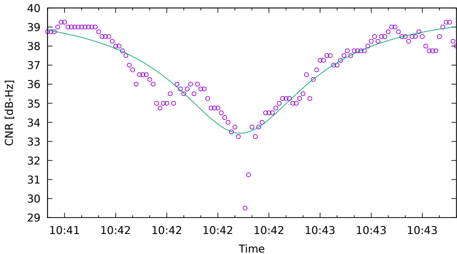
CNR fit for G19 on XiaomiMi8 - drive 2 (DOY263)
