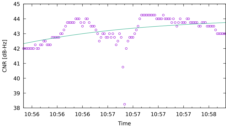
CNR fit for G21 on XiaomiMi8 - drive 10 (DOY263)
