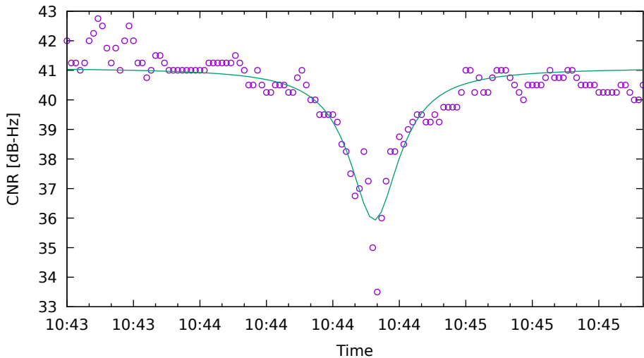
CNR fit for G21 on XiaomiMi8 - drive 3 (DOY263)
