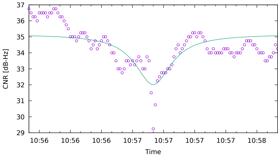
CNR fit for G22 on XiaomiMi8 - drive 10 (DOY263)
