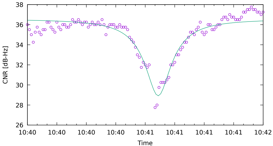
CNR fit for G31 on XiaomiMi8 - drive 1 (DOY263)
