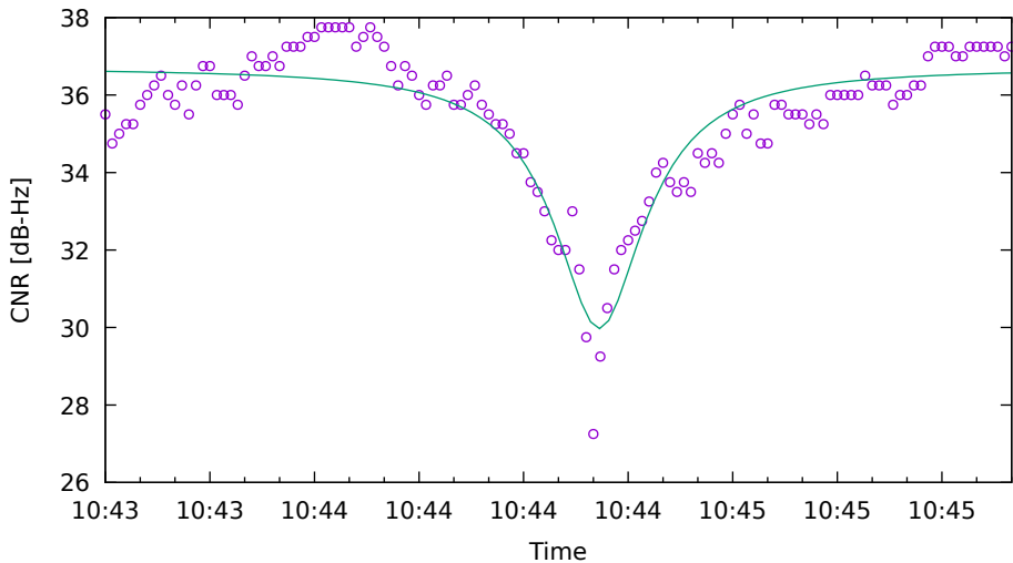
CNR fit for G31 on XiaomiMi8 - drive 3 (DOY263)
