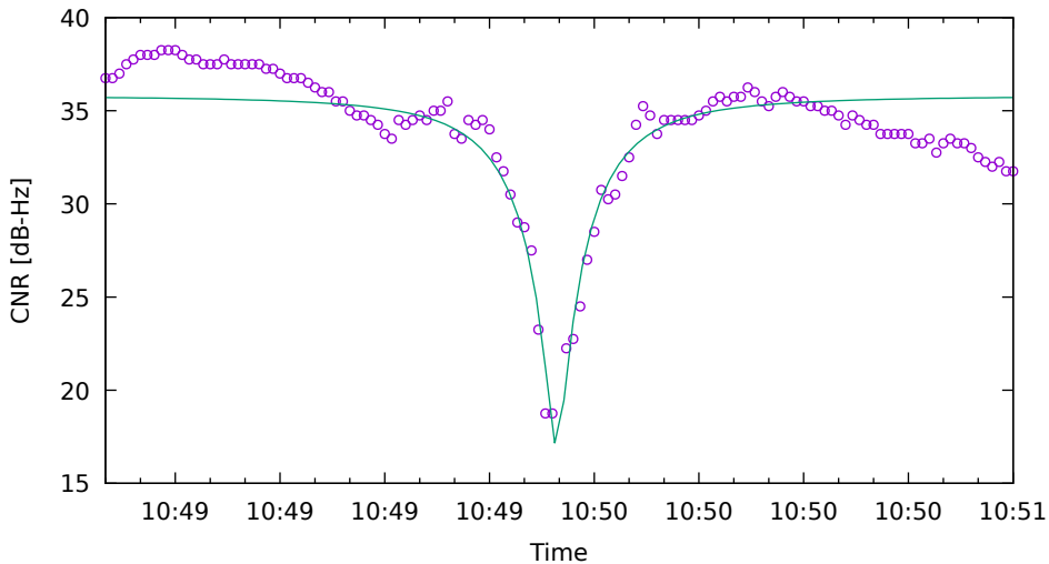
CNR fit for G31 on XiaomiMi8 - drive 6 (DOY263)
