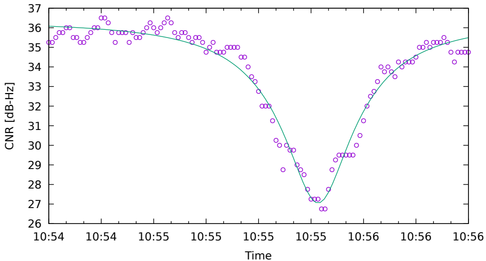
CNR fit for G31 on XiaomiMi8 - drive 9 (DOY263)
